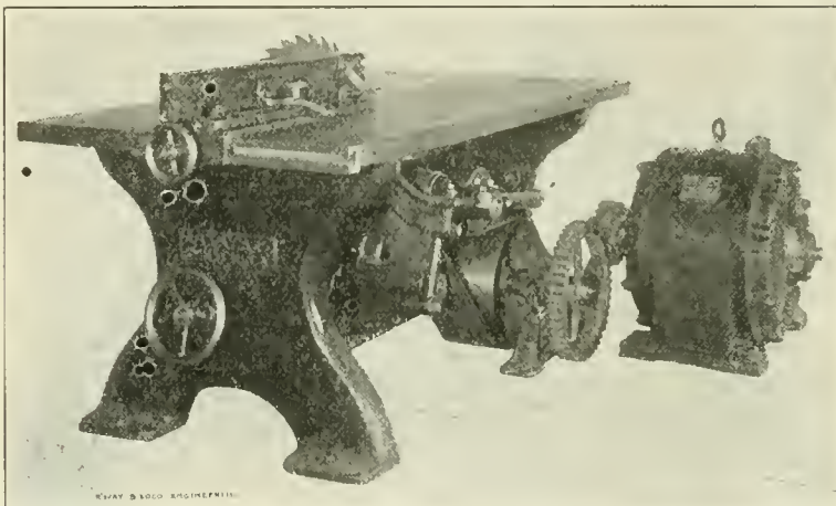
LARGE SIZE CAR RIPPING-SAW, MOTOR DRIVEN.
